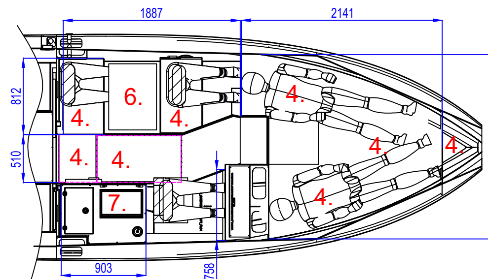
Aaltomarine 725 Fishmaster
